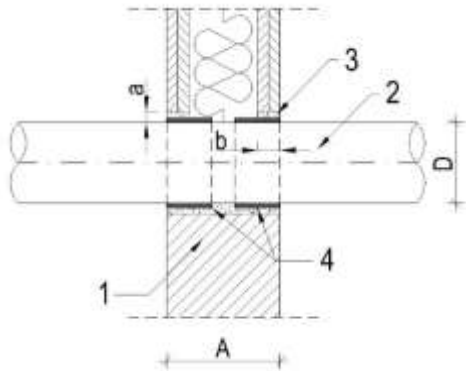
Fig. B12. Plastic pipe, MLC pipe and composite pipe (without insulation) penetration seals made with use of double row of INTU FR WRAP or INTU FR WRAP L in flexible or rigid wall.
