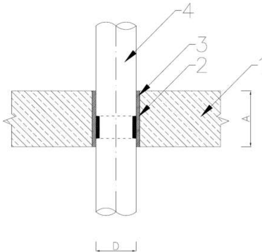
Fig. F7. Plastic pipe without insulation penetration seals made with use of INTU FR SLEEVE in rigid floor
