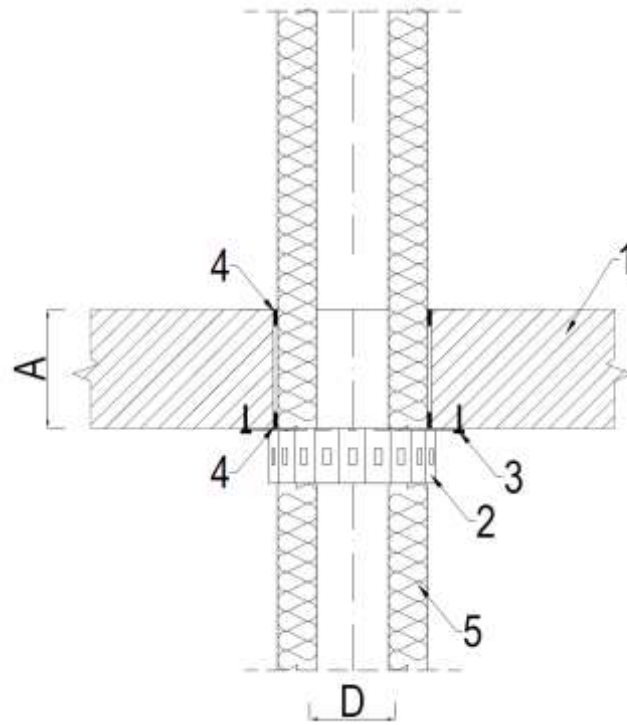
Fig. F6. Metal pipe with insulation penetration seal made with use of INTU FR COLLAR L in rigid floor
