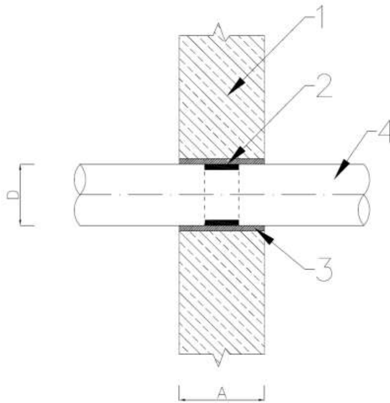
Fig. F4. Plastic pipe without insulation penetration seals made with use of INTU FR SLEEVE in rigid wall
