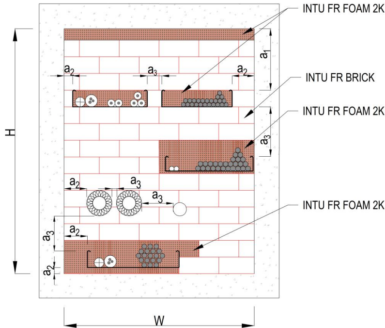
Fig. 7 Mixed penetration seal - minimum working clearances
