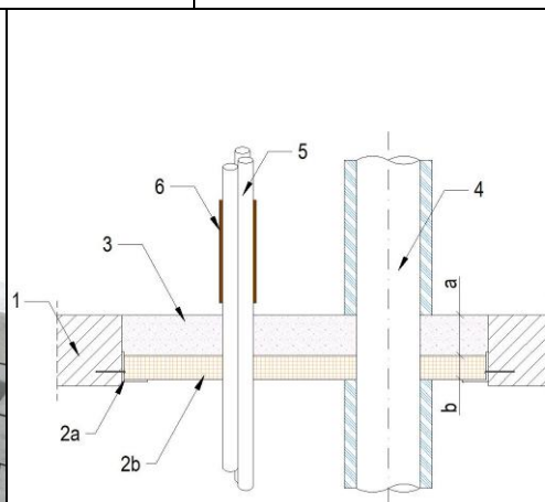
Fig. 3 Isolated non-combustible pipes and cable bundles in floor
